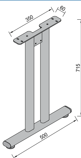
MADRID BASIC 500 mm
