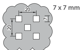
Perforation: / Perforation:
