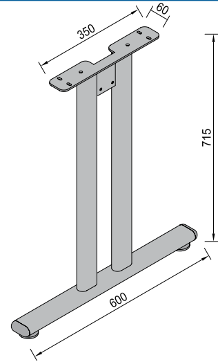
MADRID BASIC 600 mm
