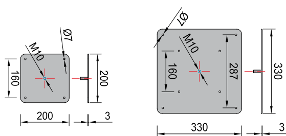
Support plate MAXIS / Tragplatte MAXIS
