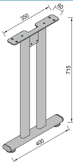
MADRID BASIC 400 mm
